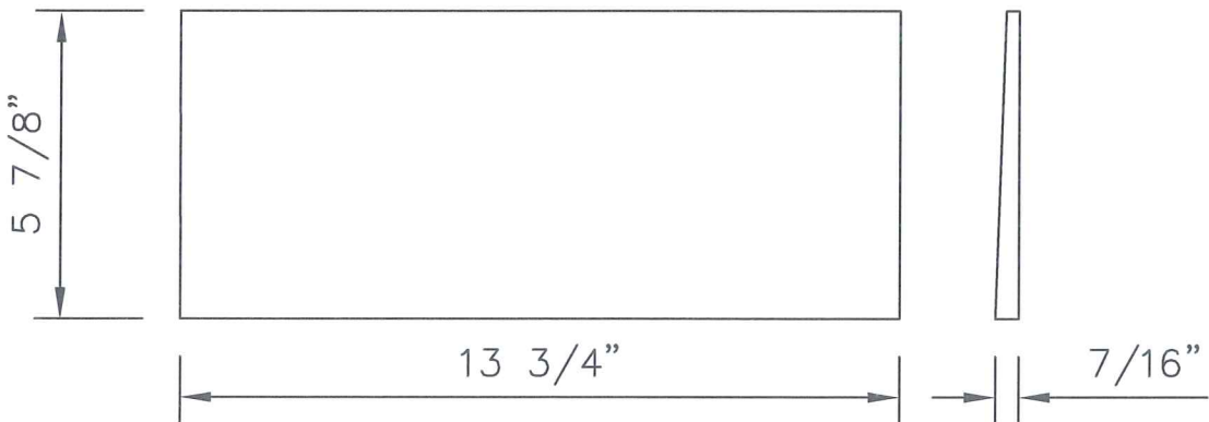
EAVE STARTER
