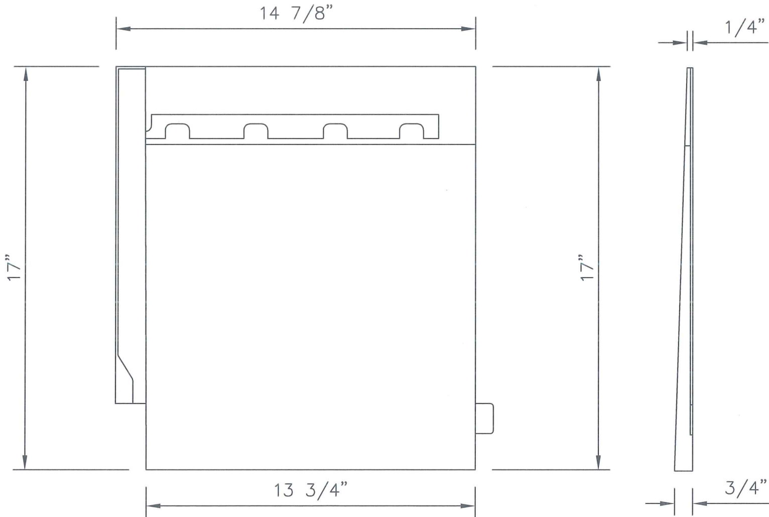
NATURA SLATE COMPOSITE SHINGLE
