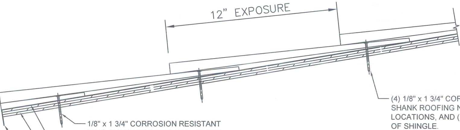
SIDE VIEW
